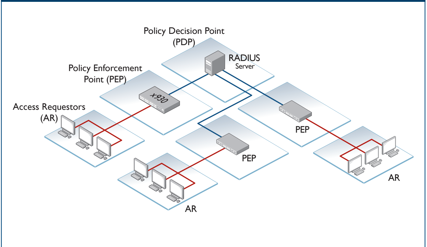
Figure 3: NAC Integration
