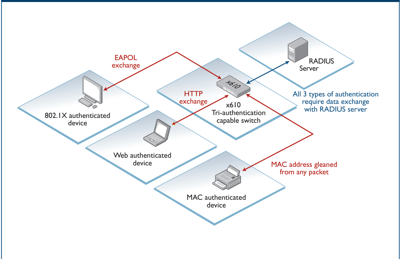
Figure 2: Tri-authentication
